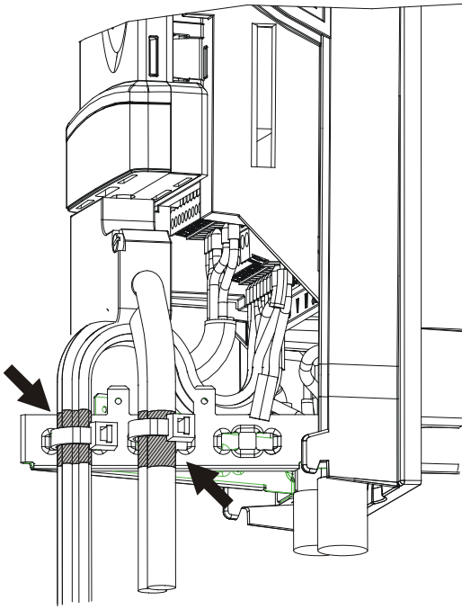
Figure 8: Earthing of signal cable screens using the grounding bracket
