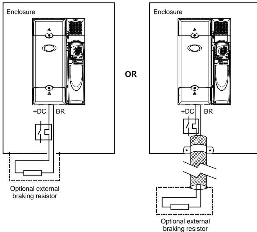
Figure 6: Screening of braking circuit
