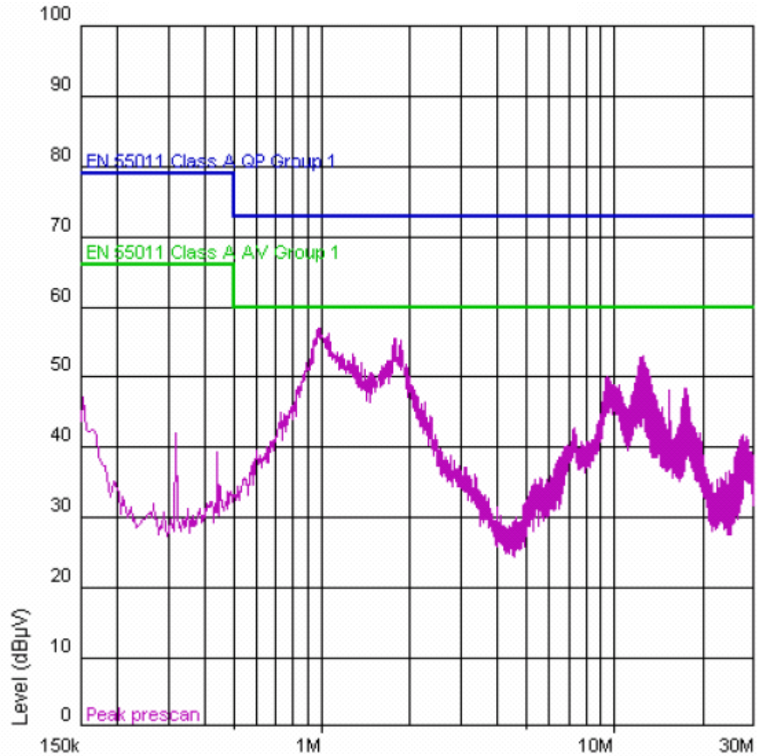
Figure 11: Example conducted emission plot (5401, 20m cable, 3kHz switching frequency)
