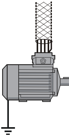
Figure 5: Connecting the motor cable shield at the motor
